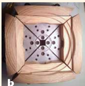
b Jumbo, flat, or Cole chuck jaws outfitted with custom-turned extension blocks can hold the disk blank. These accessory jaws are screwed in from the back of the chuck jaws but could also be screwed from the front with countersunk holes.
