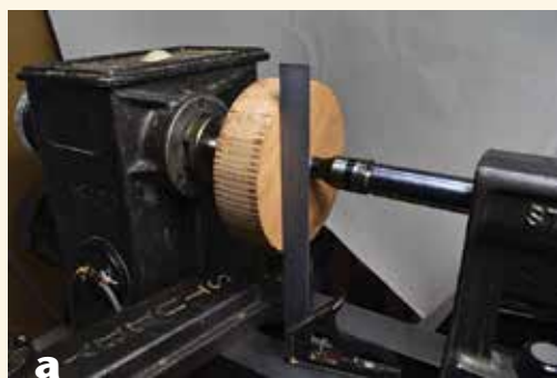
a With the tailstock live center registered on the center point of one face, square the blank to the bed ways to locate the center point on the back (headstock) side.
